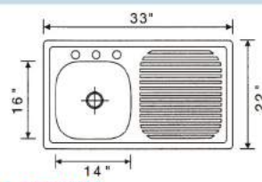
481-3322BD Stainless steel sink Overall Size: 33x22" Big bowl: 14x16x6" 5pc/18.5kg/19.5kg/1.54'
