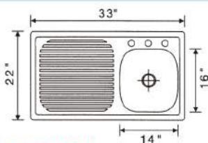
481-3322BDR Stainless steel sink Overall Size: 33x22" Big bowl: 14x16x6" 5pc/18.5kg/19.5kg/1.54'
