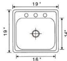
481-1919 Stainless steel sink Overall Size: 19x19" Big bowl: 16x14x6" 5pc/11kg/12kg/0.79'
