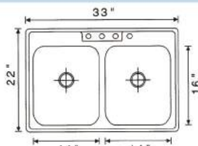
481-3322 Stainless steel sink Overall Size: 33x22" Big bowl: 14x16x6-7/8" 5pc/30kg/31kg/2.05'
