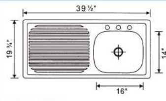
481-3920R Stainless steel sink Overall Size: 39-1/2x19-3/4" Big bowl: 16x14x6" 5pc/20kg/21kg/1.61'
