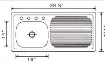
481-3920 Stainless steel sink Overall Size: 39-1/2x19-3/4" Big bowl: 16x14x6" 5pc/20kg/21kg/1.61'
