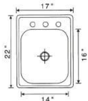
481-1722 Stainless steel sink Overall Size: 17x22" Big bowl: 16x14x6-7/8" 5pc/10kg/11kg/0.82'
