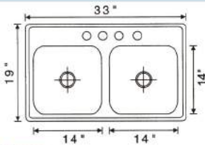
481-3319 Stainless steel sink Overall Size: 33x19" Big bowl: 14x14x6-7/8" 5pc/25.5kg/26.6kg/1.5'
