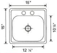
481-1515 Stainless steel sink Overall Size: 15 x 15" Big bowl: 12-1/4x10-1/2x5-1/2" 5pc/22.5kg/23.5kg/1.54'
