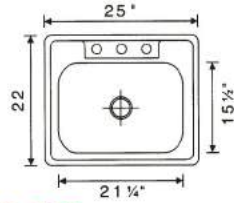
481-2522 Stainless steel sink Overall Size: 25x22" Big bowl: 21-1/4x15-1/2x6-7/8" 5pc/20kg/21kg/1.31'
