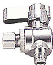
183-105 1/4-turn ball valve 1/8"MIP x 1/4" O.D. 150pc/18/19/0.7'
