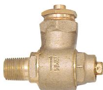
Brass swivel pattern ferrule With single outlet 30-011-12 : 1/2" 50pc/23kg/24kg/0.5' 30-011-34 : 3/4" 40pc/20kg/21kg/0.5'
