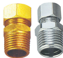
Straight male adapter 19-008-3838 3/8" MIP x 3/8" OD 500pc/21kg/22kg/0.5' 19-008-1238 1/2" MIP x 3/8" OD 500pc/22kg/23kg/0.5'
