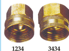
Brass fittings 19A-023-1234 : 1/2" FIP X 3/4" FNH 50/bag 300pcs/18.5kg/19kg/0.5' 19A-023-3434 : 3/4" FIP X 3/4" FNH 50/bag 300pcs/20kg/21kg/0.5'
