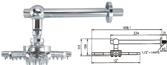
24A-023 C.P. radiate rain Shower W/shower arm 24A-023-6 6" 12pc/13.3kg/14.3kg/1.2' 24A-023-12 12" 10pc/18kg/19kg/2'
