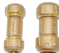
32A-014 Brass compression coupling Size: 1/2" & 3/4" 1/2": 100pc/15.7kg/16.5kg/0.4' 3/4": 100pc/22.5kg/23.5kg/0.6'
