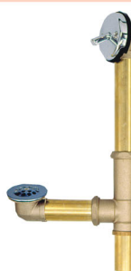
20-002 1-1/2" Trip lever waste and overflow 12pc/17kg/19kg/1.6'
