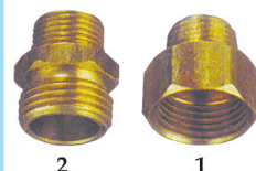
Brass fittings 19A-022-1 1/2" MIP X 3/4" FNH 300pcs/19kg/19.5kg/0.5' 19A-022-2 1/2" MIP X 3/4" MNH 300pcs/17kg/17.5kg/0.5'
