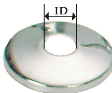
Flange for angle valve 19-011-38 3/8" ID: 17mm 19-011-12 1/2" ID: 21mm 1000pc/9kg/10kg/1.3'
